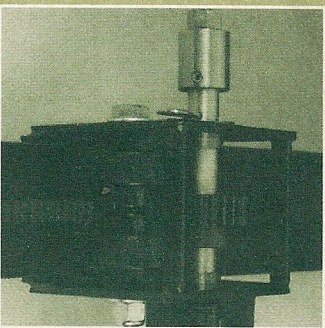
Our high quality, low friction, rack and gear electric slide out system features fast, super quiet operation. There are only a few working parts, making maintenance a breeze.
